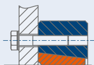
Model A: Thread in the outer ring
